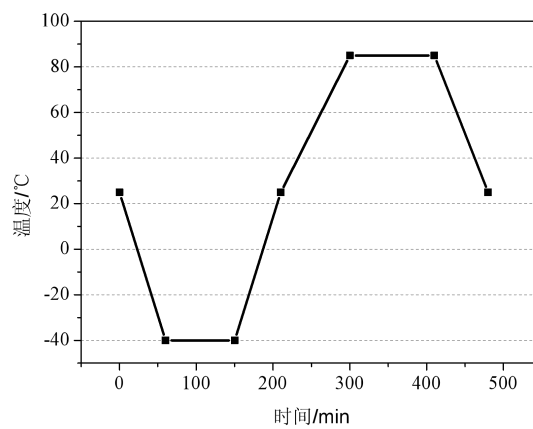
Fig 2. Schematic diagram of temperature cycle
